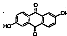
ANTHRAFLAVIC ACID
